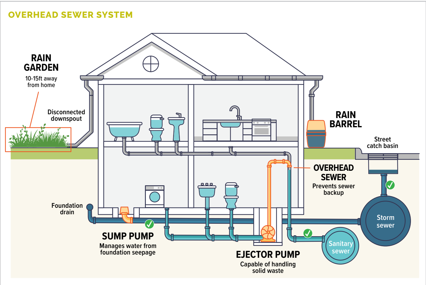
Diagram of an overhead sewer replacement. Note: The above drawing is not to scale and is for illustrative purposes only. Source: Greenprint Partners
