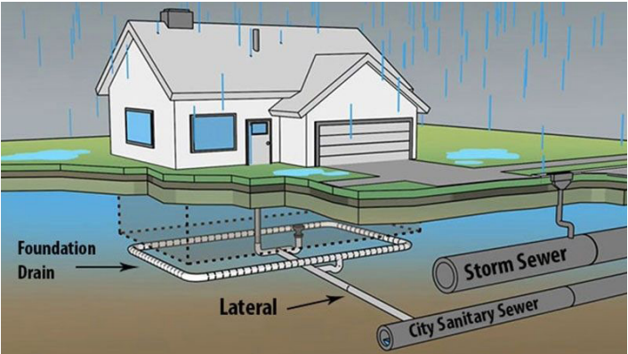
Diagram of a separated sewer system under a residence. Source: MMSD
